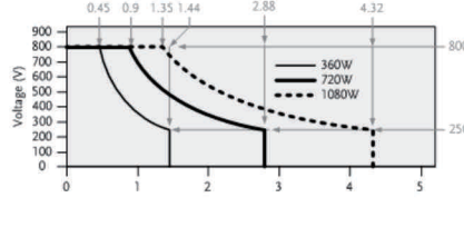
PSW 800V Series Operating Area
