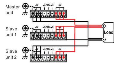
Parallel Connection
