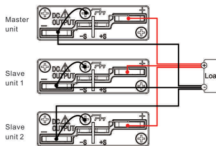
Parallel Connection
