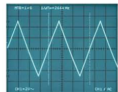
Frequency Measurement
